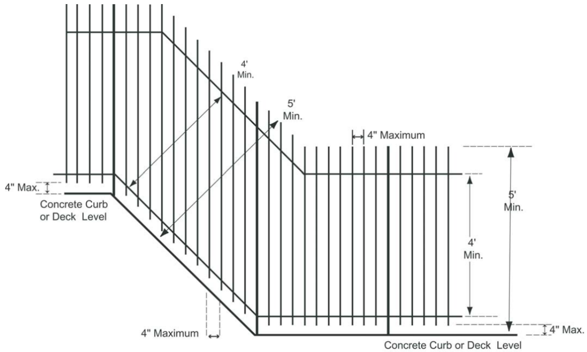
Figure 31B-5: Effective Fencing Height
