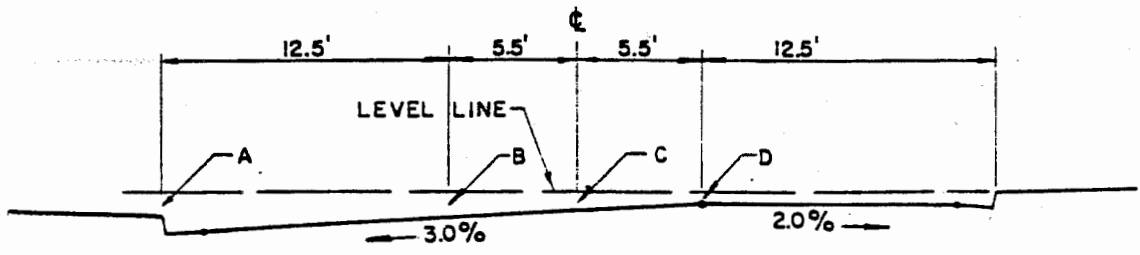
TYPICAL SECTION TILT
