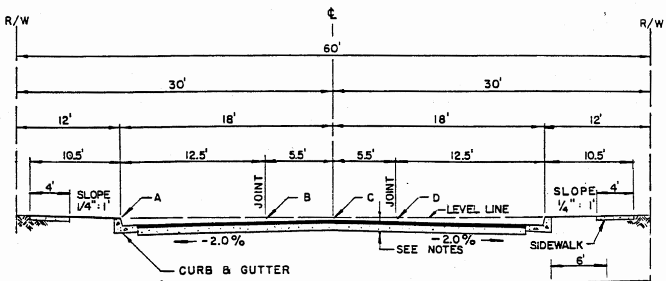
TYPICAL SECTION LEVEL
