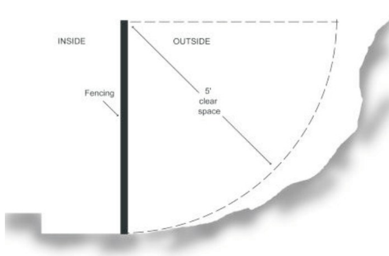
Figure 31B-5: Effective Fencing Height
