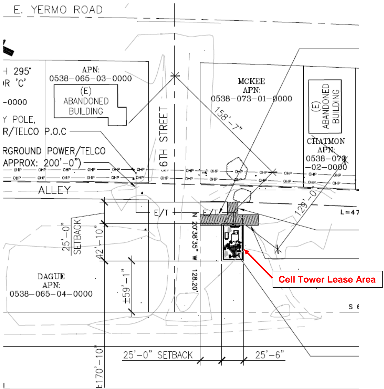
Figure 3 Area Site Location and General Project Layout
