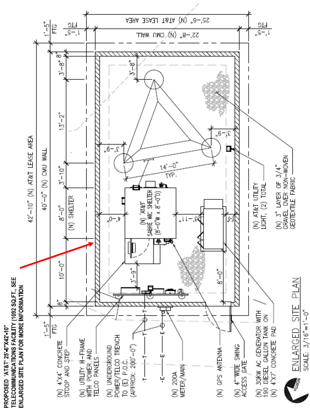
Figure 4 Site Plan
